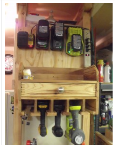
Charging Station
